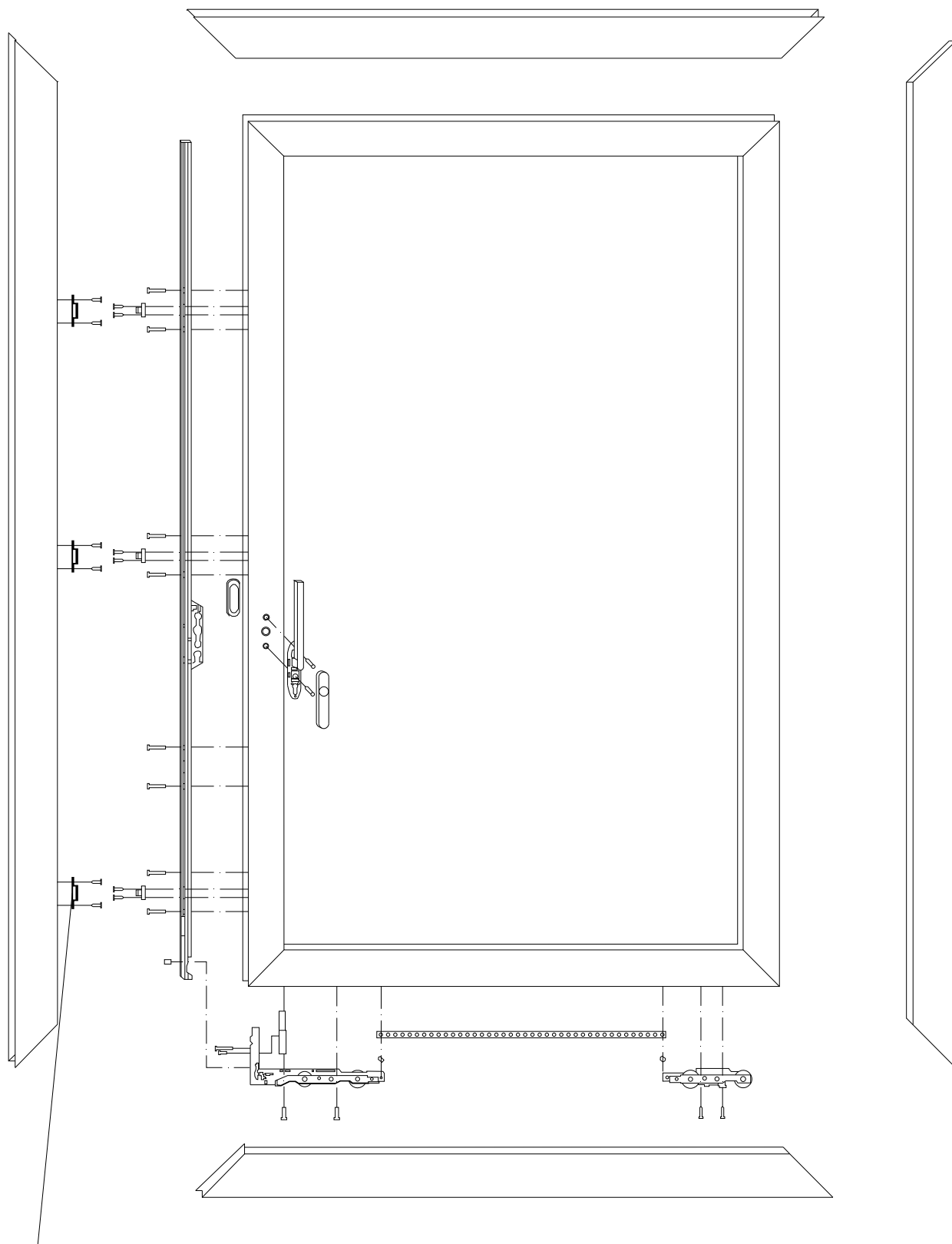
CERRADERO PERIMETRAL
